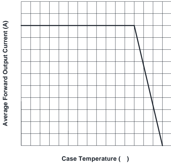
FIG1:Io-Tc Curve
